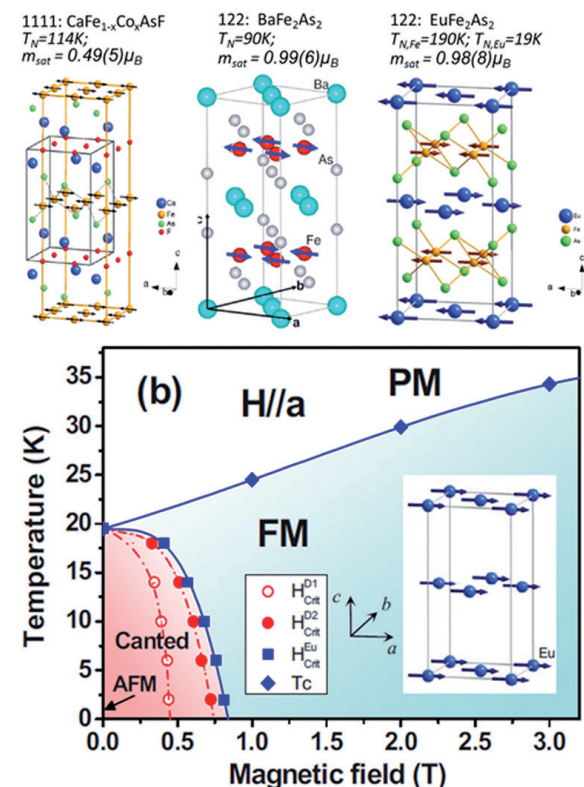
Fig. 1: Top: Zero field, low temperature magnetic structures of some parent compounds of iron based high temperature superconductors as determined by neutron diffraction. Bottom: Magnetic phase diagramme for the compound \text{EuFe}_2\text{As}_2 with magnetic field applied along the a axis (only the Eu spin moments are plotted).
