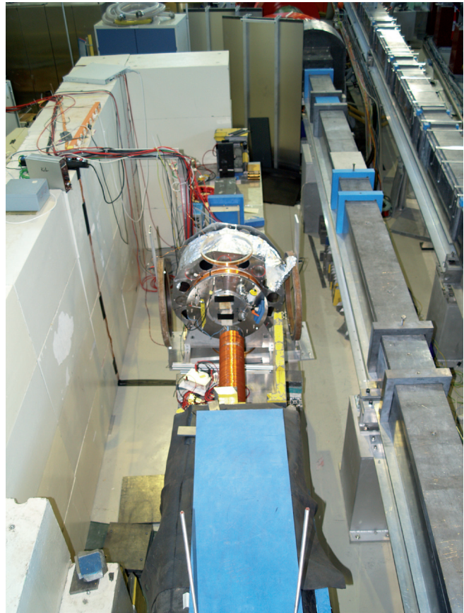
Fig. 3: Fission chamber at NL1 with surrounding coincidence detectors.
