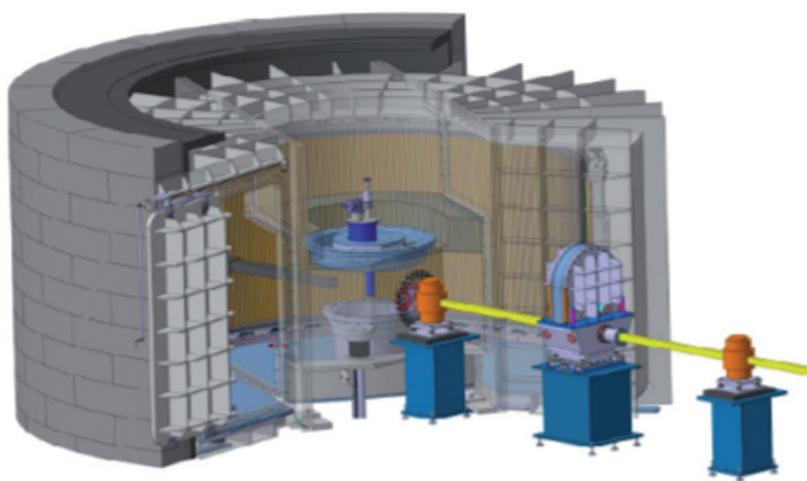
Fig. 4: Schematics of the future thermal Time-of-Flight Spectrometer with Polarization Analysis TOPAS.
