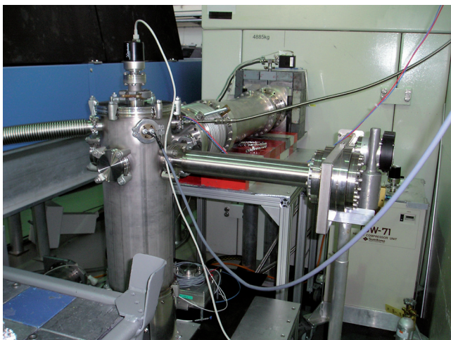
Fig. 4: UCN cryo converter partly dismantled.
